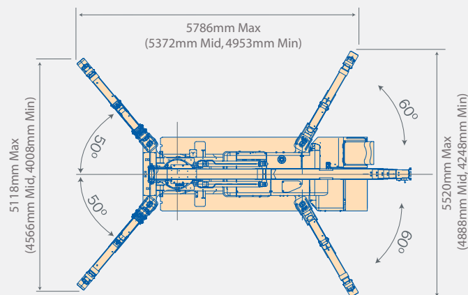
Diagram shows outriggers at maximum position
